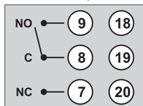
Output-2 / Output-3 Relay
