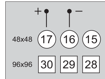
Figure 10.2(c) mA / mV / V Input
