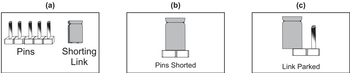
Figure 11.5 : Jumper Settings
