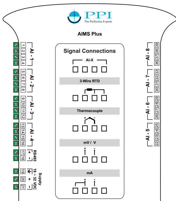
4 Channel Module
