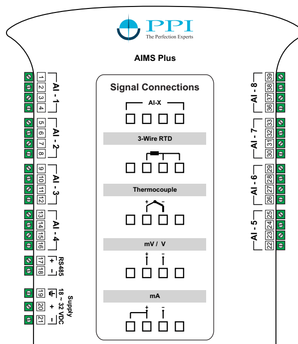
8 Channel Module
