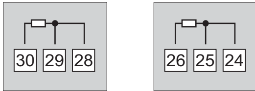
Temperature Input
