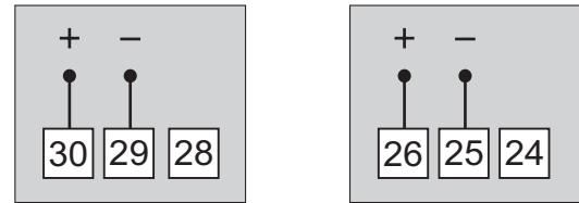
Temperature Input
