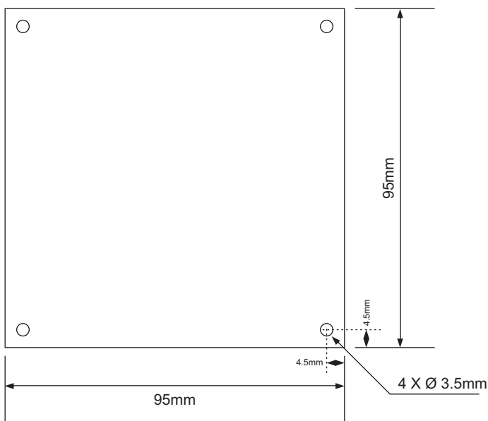
Figure 1.2 : Control Board
