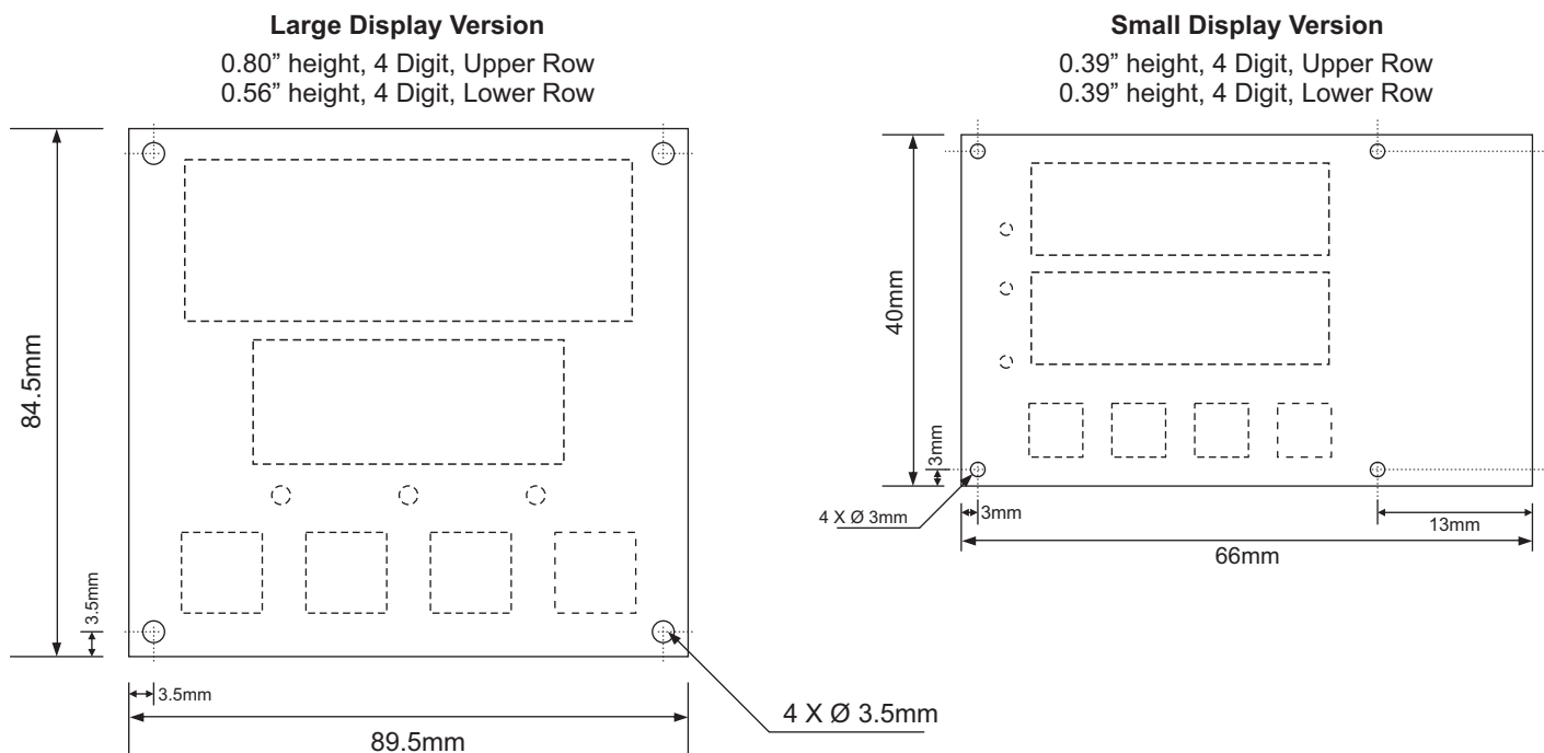
Figure 1.1 : Display Boards
