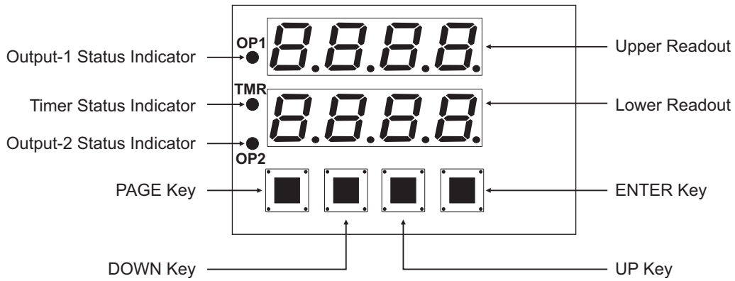
Figure 2.1(a) : Small Display Board
